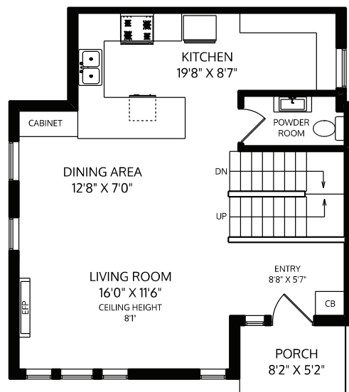
MAIN FLOOR
