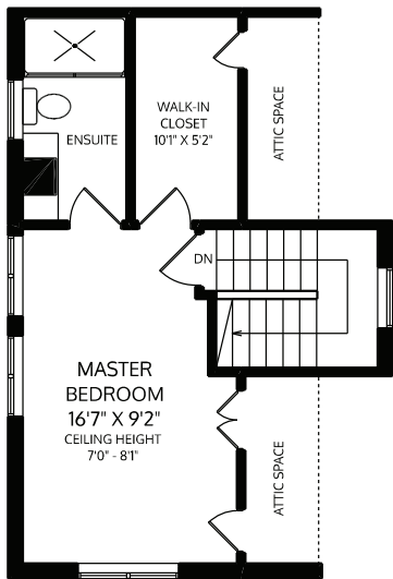
UPPER FLOOR
