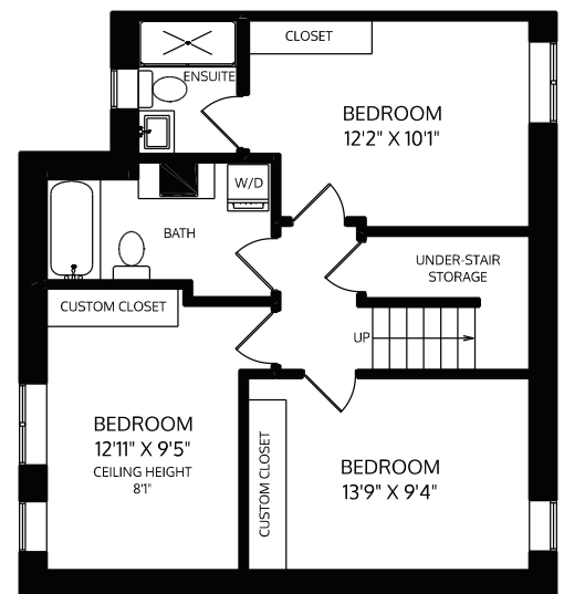
LOWER FLOOR
